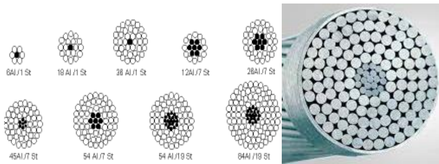
Figura 3-4 Conductor ACSR.
